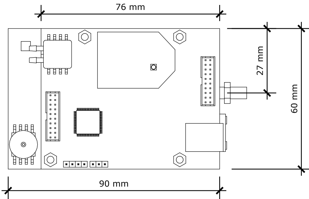
SkyCircuits SC2 (Without Enclosure) Drawing Scale 1:1 Mass: 85g
